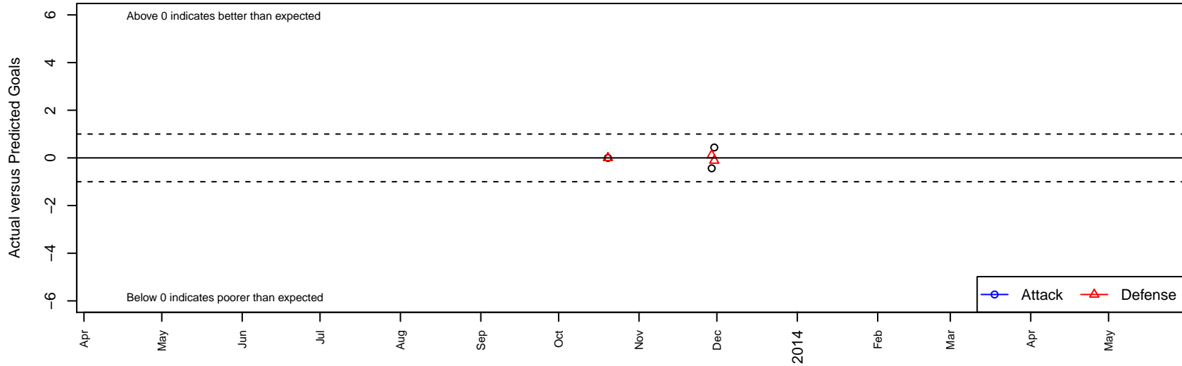
Legends FC South B97 Dots are actual minus expected GF (blue circles) and GA (red triangles). Blue line is smoothed change in attack strength. Red is smoothed change in defense strength.
